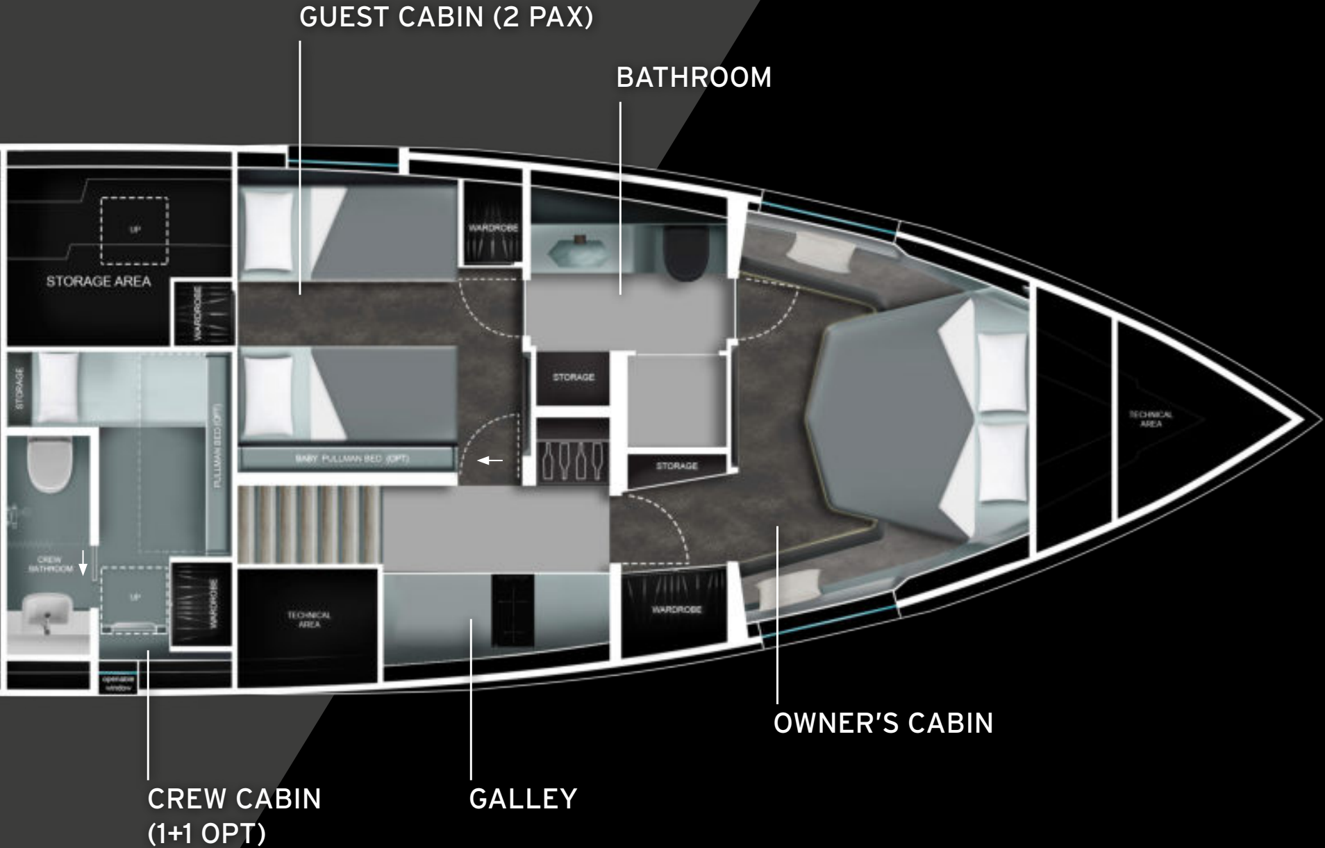
TWO CABINS LAYOUT 4+1 GUEST
